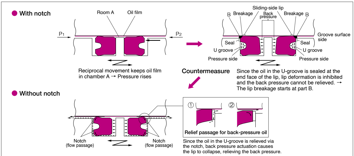
〈Fig. H-25〉 Mechanism of package failure due to pressure build-up and countermeasures
