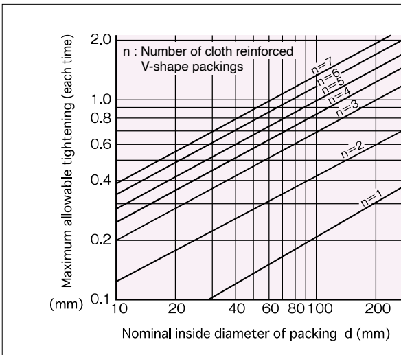
(Fig. F-32) Max. allowable tightening
