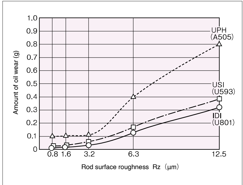
〈Fig. H-4〉 Rod Surface Roughness and Amount of Wear
