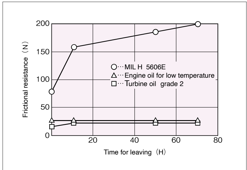
〈Fig. H-13〉 Result of measurement of initial frictional resistance
