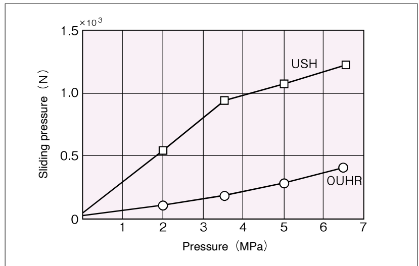
〈Fig. H-9〉 Frictional resistance and pressure
